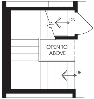
PARTIAL MAIN FLOOR FOR OPTIONAL LOFT
