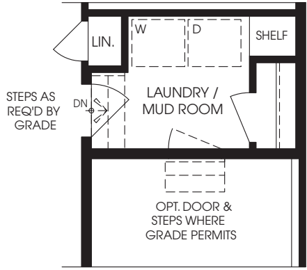
PARTIAL MAIN FLOOR FOR OPTIONAL LOFT
