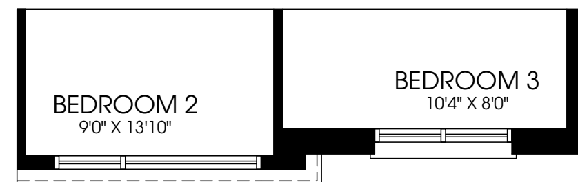
PARTIAL SECOND FLOOR ELEVATION 'B2'
