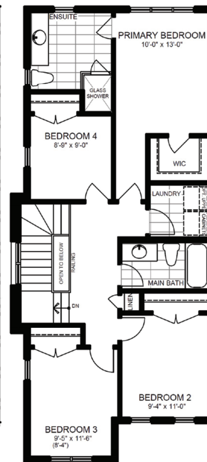
ALTERNATE 4 BEDROOM SECOND FLOOR PLAN ELEVATION 'A4' CORNER
