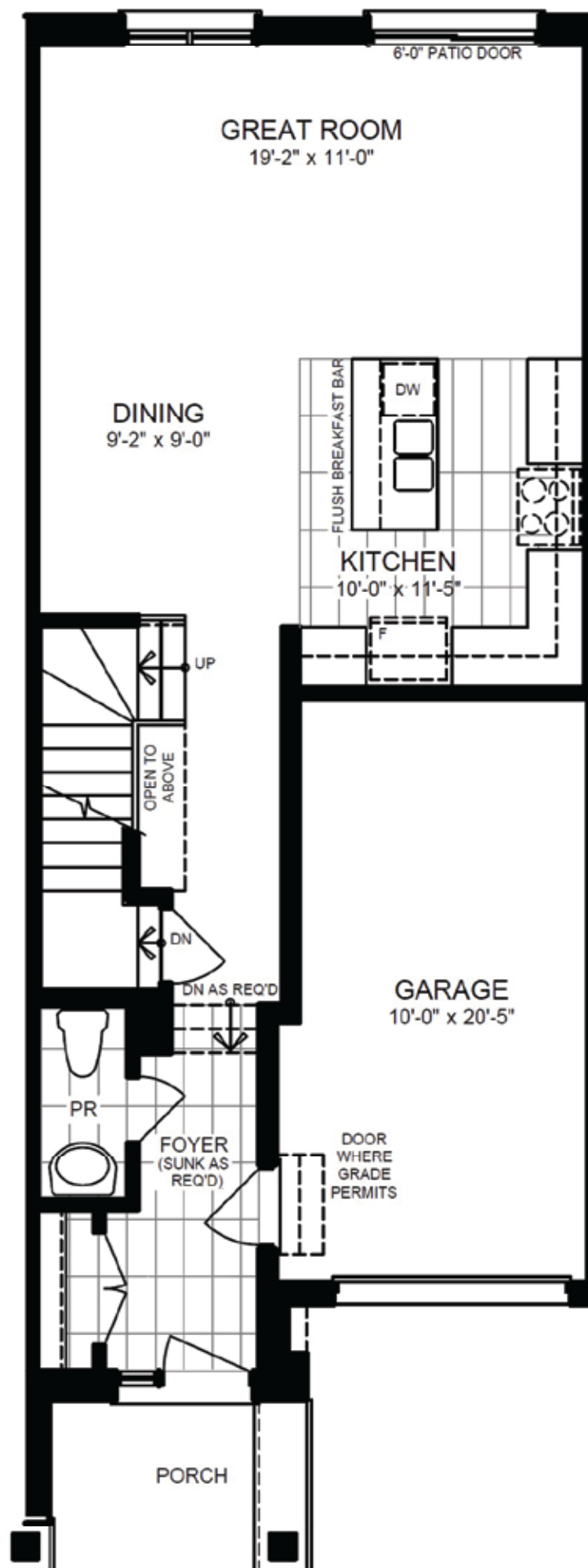
MAIN FLOOR PLAN ELEVATION 'A1' & 'A2'
