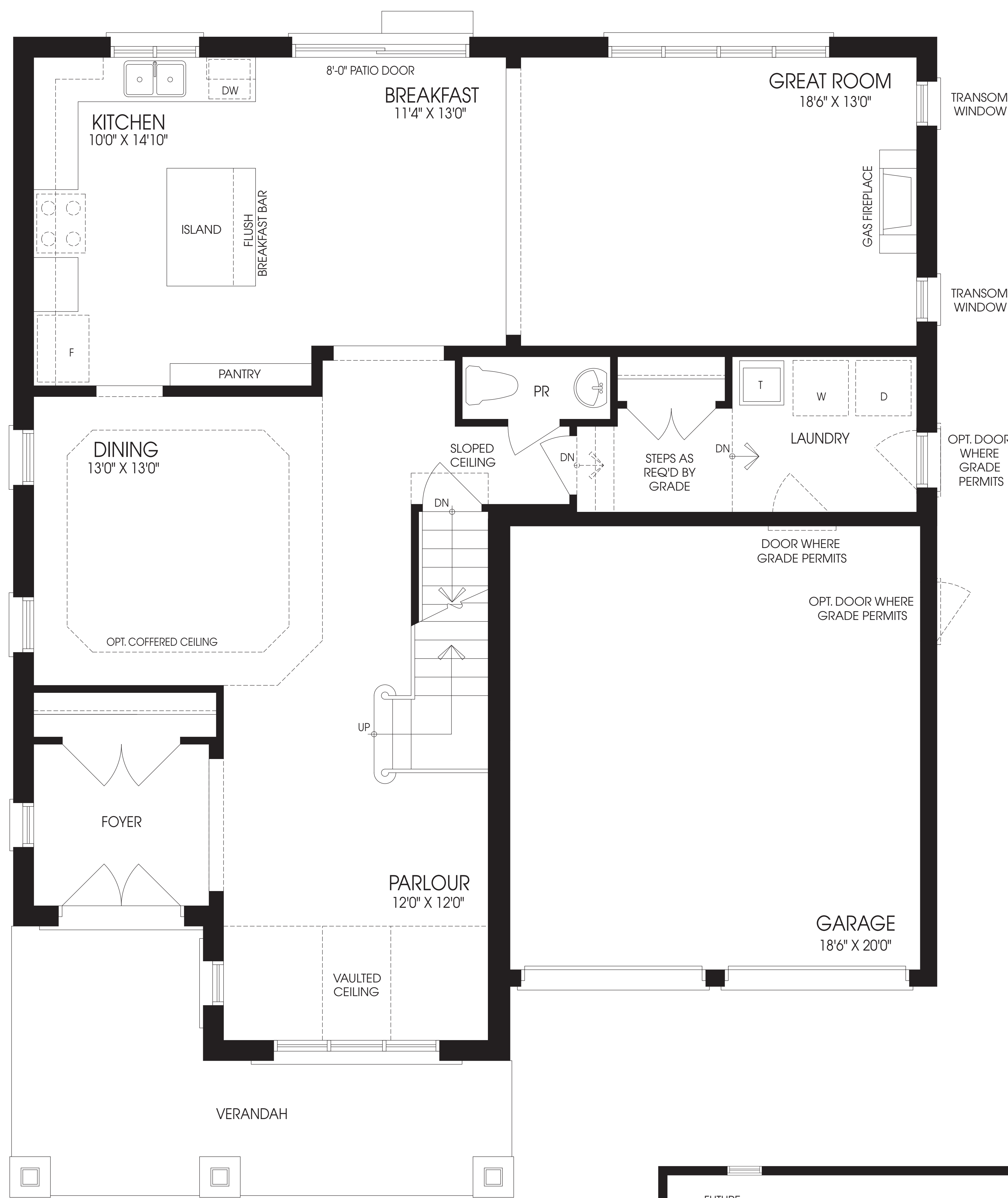
MAIN FLOOR ELEVATION 'B'
